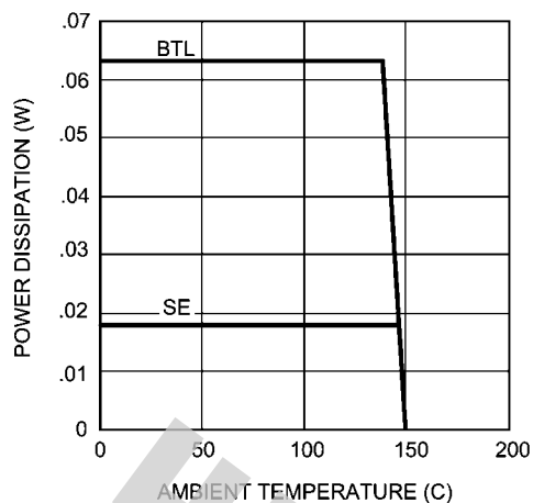
Power Derating Curve V_{DD} = 1.5V
