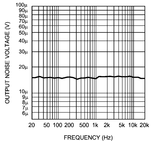
Noise Floor V_{DD} = 1.5V , R_L = 8\Omega BW < 80kHz , BTL Output
