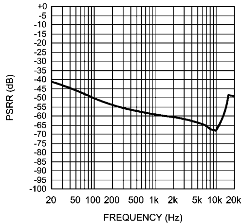
Power Supply Rejection Ratio V_{DD} = 1.2V , V_{RIPPLE} = 200mV_{PP} R_L = 8\Omega , BTL Output Input Terminated into 10\Omega
